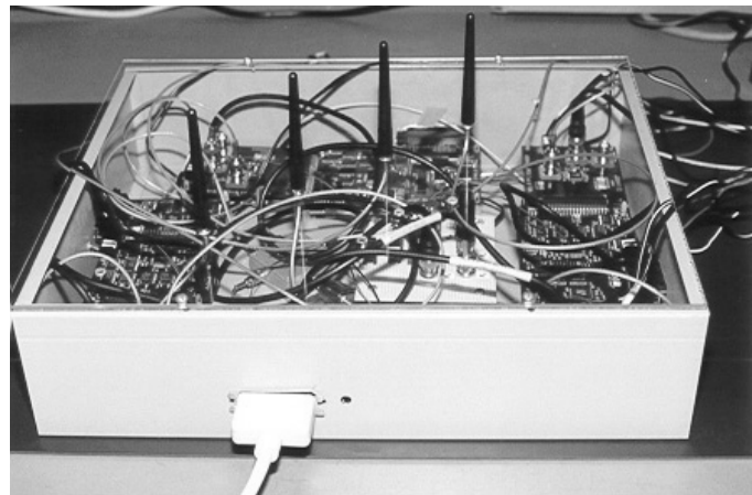
Fig. 2. Photograph of receiving basestation
