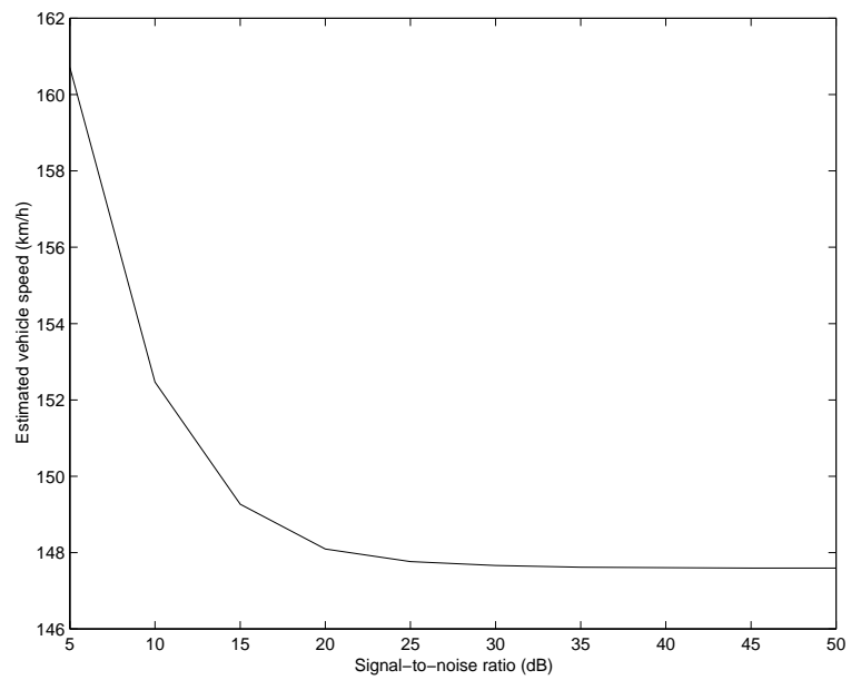
Figure 3.21: Simulation results of actual vehicle speed of 150 km/h in presence of two-term mixture Gaussian noise
