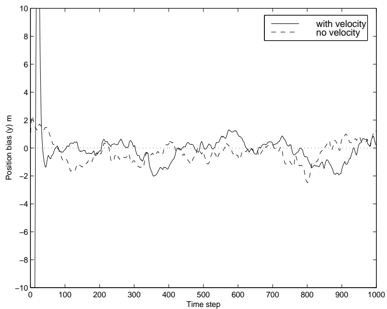
Figure 5.7: y position bias, mobile velocity: 5 km/h, position measurement error: 20 m
