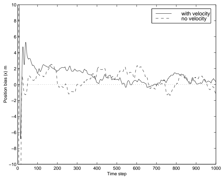
Figure 5.17: x position bias, mobile velocity: 20 km/h, position measurement error: 20 m
