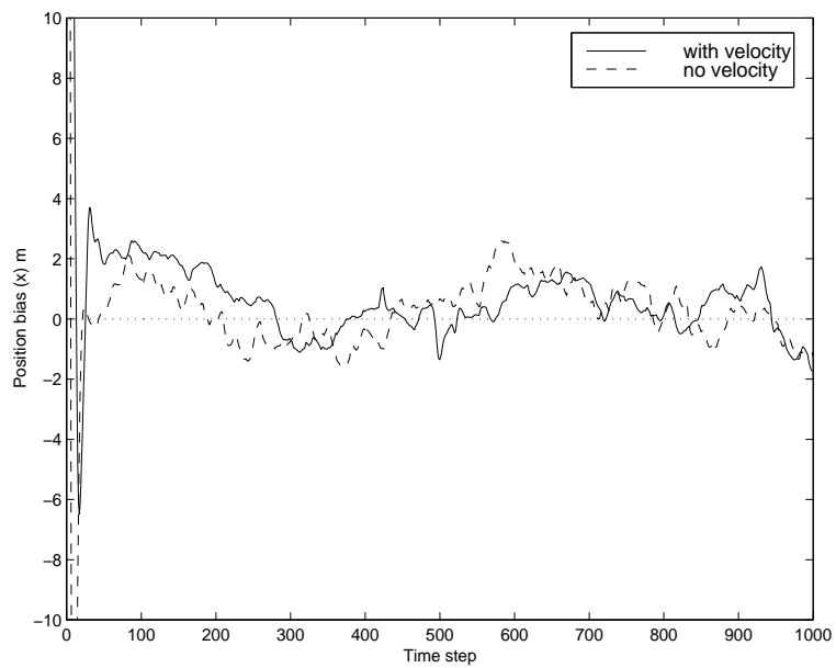
Figure 5.5: x position bias, mobile velocity: 5 km/h, position measurement error: 20 m
