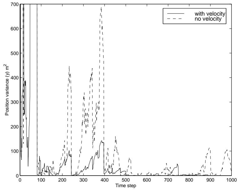
Figure 5.38: y position variance, mobile velocity: 50 km/h, position measurement error: 100 m
