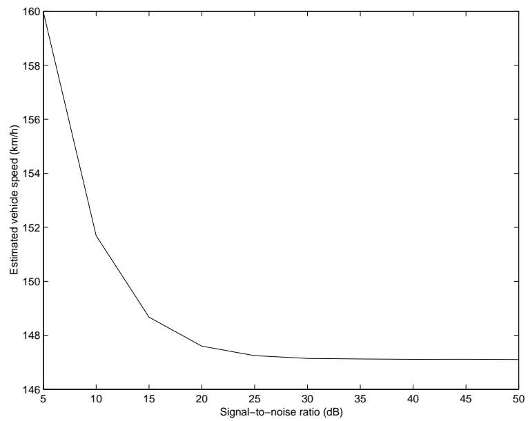
Figure 3.15: Simulation results of actual vehicle speed of 150 km/h in presence of additive Gaussian noise
