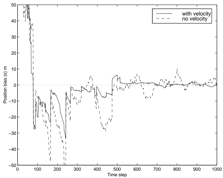
Figure 5.37: x position bias, mobile velocity: 50 km/h, position measurement error: 100 m
