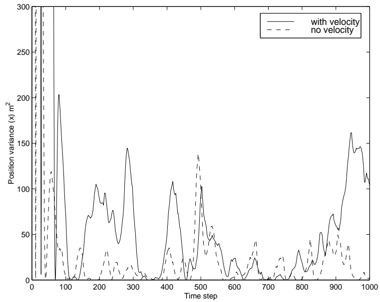
Figure 5.12: x position variance, mobile velocity: 5 km/h, position measurement error: 100 m
