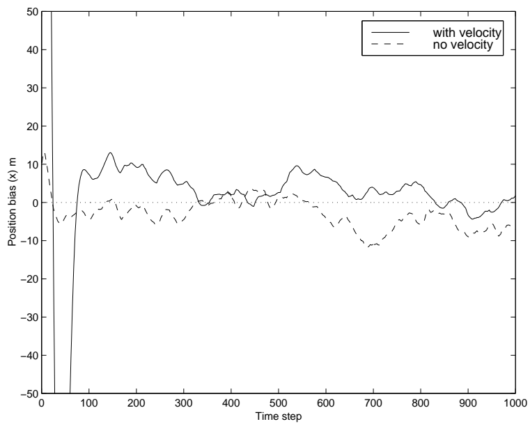
Figure 5.25: x position bias, mobile velocity: 20 km/h, position measurement error: 100 m
