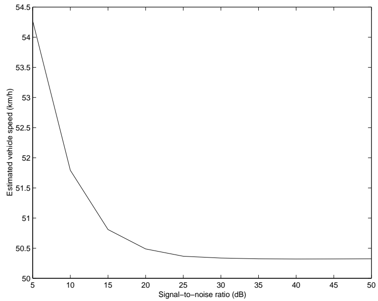
Figure 3.11: Simulation results of actual vehicle speed of 50 km/h in presence of additive Gaussian noise
