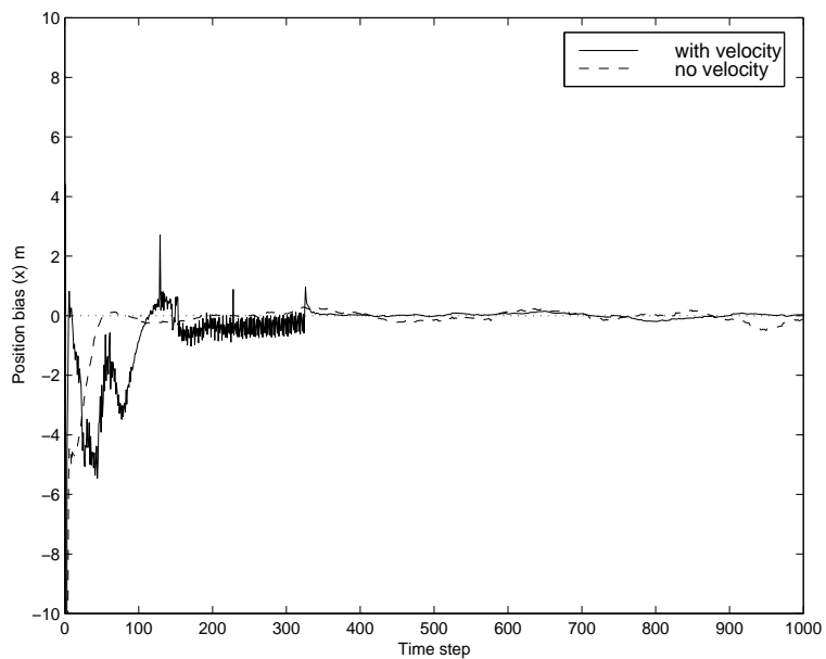
Figure 5.45: x position bias, mobile velocity: 100 km/h, position measurement error: 40 m
