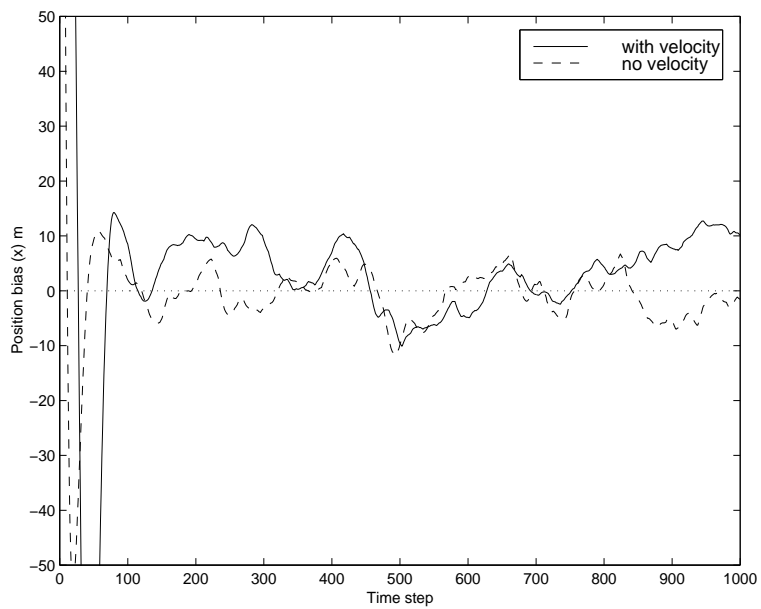
Figure 5.13: x position bias, mobile velocity: 5 km/h, position measurement error: 100 m
