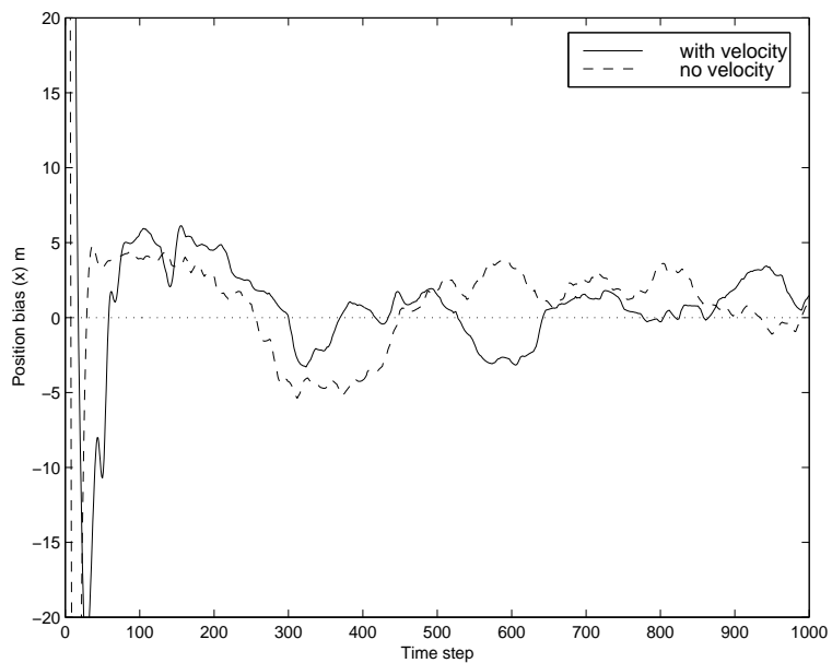
Figure 5.21: x position bias, mobile velocity: 20 km/h, position measurement error: 40 m
