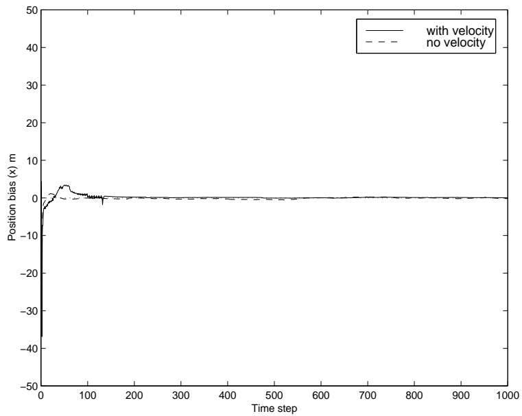
Figure 5.49: x position bias, mobile velocity: 100 km/h, position measurement error: 100 m
