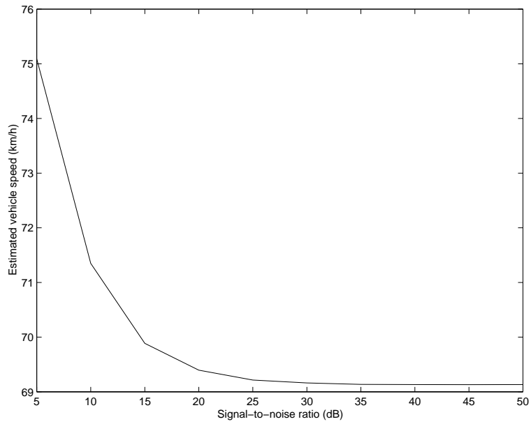
Figure 3.12: Simulation results of actual vehicle speed of 70 km/h in presence of additive Gaussian noise
