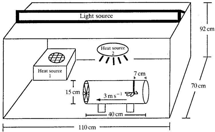
Fig. 1. The experimental apparatus for intact animal experiments. Experiments were carried out within a shielded cage. Animals were tethered and flown in a wind-tunnel with a wind speed of 3 \text{ m s}^{-1} . To increase ambient temperature, a small room heater with a fan was used (heat source 1) and to increase thoracic temperature at intervals during flight a 250W infrared lamp was used (heat source 2).
