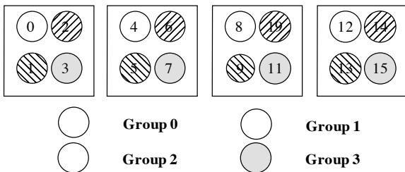
Figure 4. Group structure for 4-group all-gather on a 4-node, 16-core cluster.
