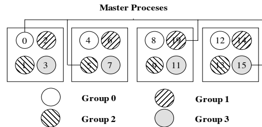
Figure 2. Group structure for gather-based all-gather on a 4-node, 16-core cluster.
