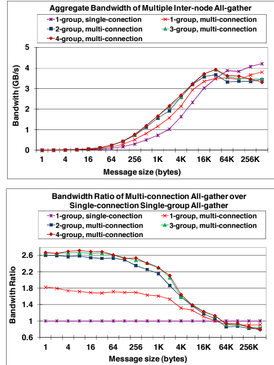
Figure 1. Aggregate bandwidth of multiple independent all-gather operations.
