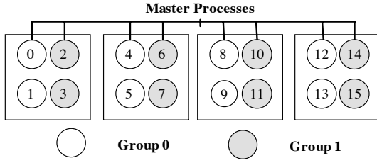
Figure 3. Group structure for 2-group all-gather on a 4-node, 16-core cluster.
