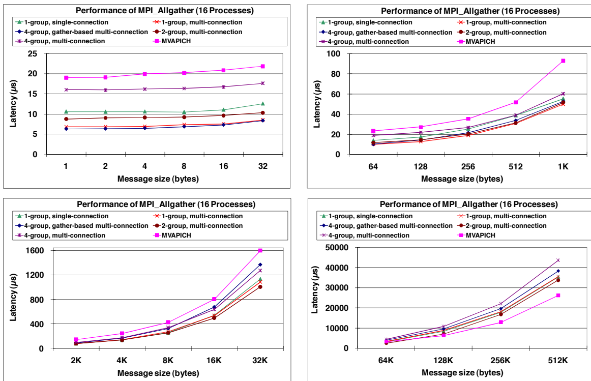
Figure 5. Performance of the proposed MPI_Allgather algorithms on a 4-node, 16-core cluster.
