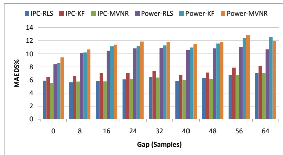
Fig. 6 Overall average of mean absolute error for different gap sizes when predicting IPC and power
