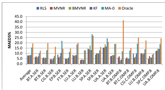
(a) MAEDS
