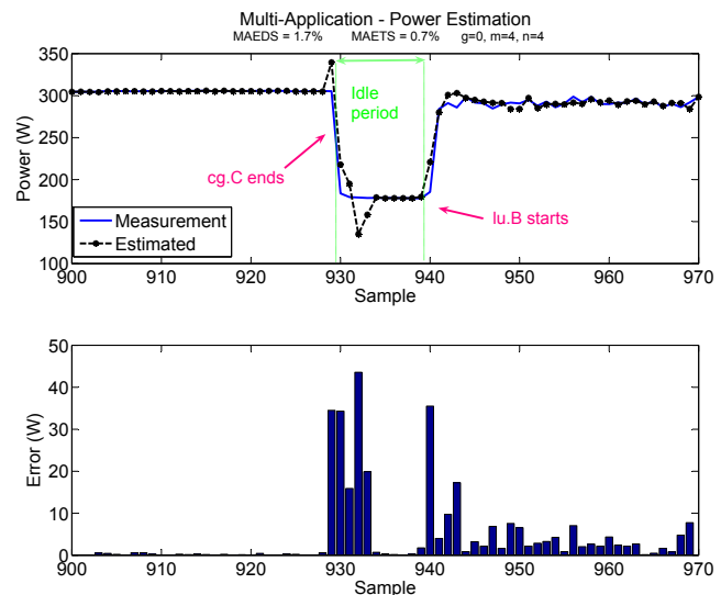
Fig. 7 Runtime power estimation of multiple applications (extreme cases: idle period, and start/end of a benchmark)
