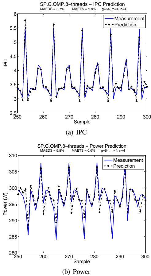
Fig. 5 IPC and power prediction for SP.C.OMP with 8 threads using RLS, gap=64 samples (i.e. 65 steps ahead)
