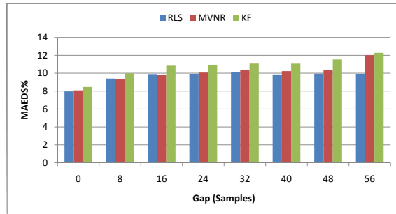
Fig. 4 Delay effect on mean absolute error using different coefficient update algorithms
